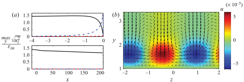
FIGURE 16. (a) Normalized spanwise r.m.s. of u (—), v (----) and w (.....) on the stagnation streamline (top) and far above the plate ( y = 15b , bottom) for free-stream \eta_y -modes with (\gamma, \beta)_j = (0, 0.36)j ( j = 1 \dots 6 ) and F = 0 . (b) Instantaneous u (colours), v and w (vectors) in the boundary layer at x = 175b ( Re_x = 4.2 \times 10^5 ) for forcing with the \eta_y -mode from figure 15.
