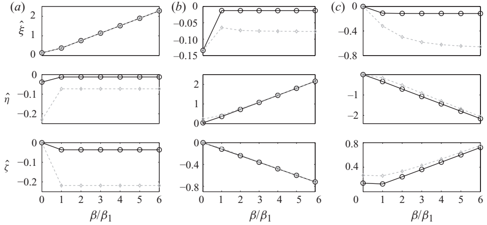
FIGURE 5. Vorticity amplitudes of inflow disturbances constructed from seven vortical modes with wavenumber (\gamma, \beta)_0 = (0.1344, 0) ; (\gamma, \beta)_j = (0.12, 0.36)j , j = 1 \dots 6 . Frequency F = 16 (black —, \circ ) and F = 96 (grey ---, \diamond ). (a) \xi -modes. (b) \eta -modes. (c) \zeta -modes.
